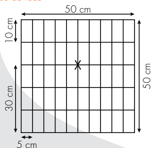
Gabion CUBIK 100x50 cm - haut. 50 cm
